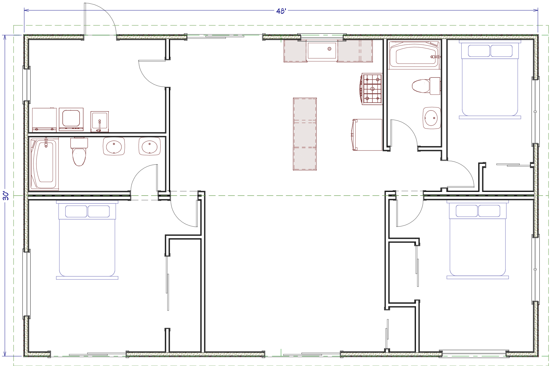
30X48 FUSION 3 BEDROOM 2 BATH 1440 SQ FT
