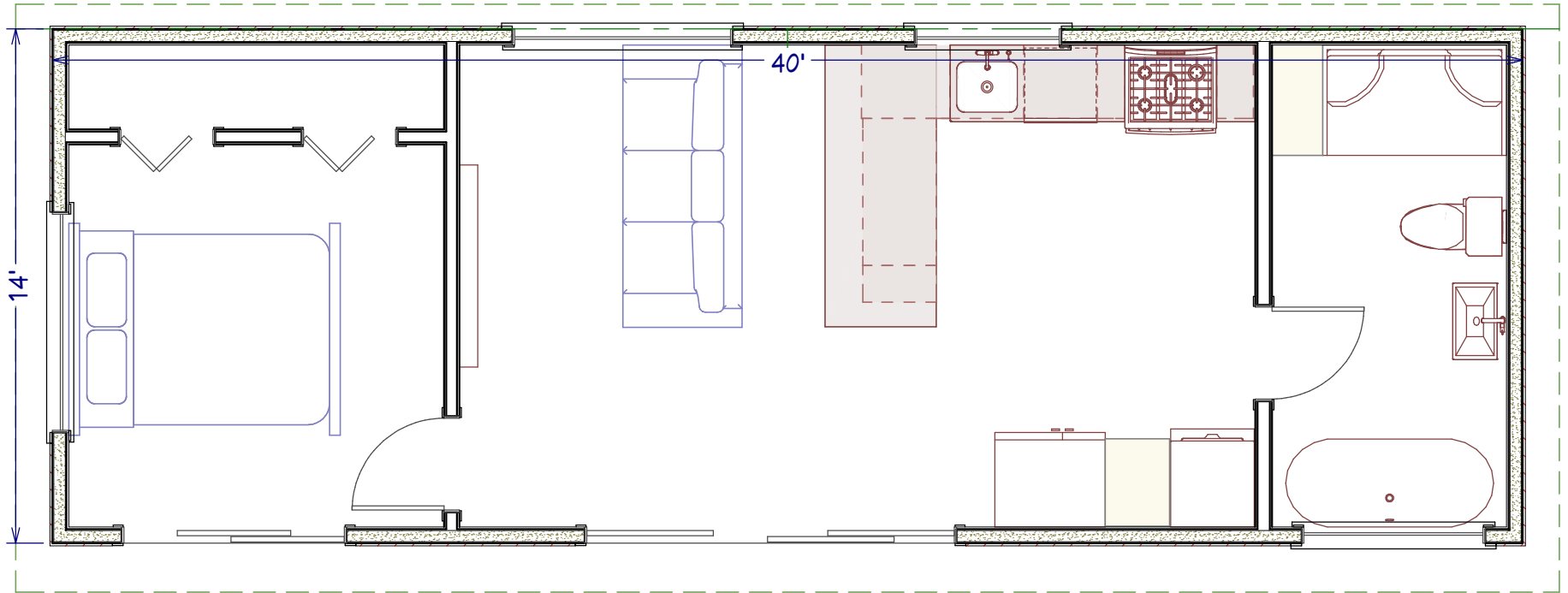
14X40 OUTLOOK 1 BEDROOM, 1 BATH 560 SQ FT
