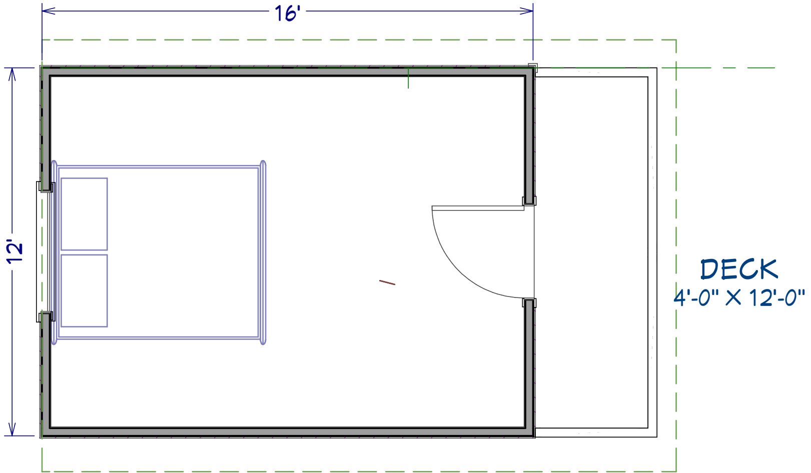
12X20 A FRAME 192 SQ FT
