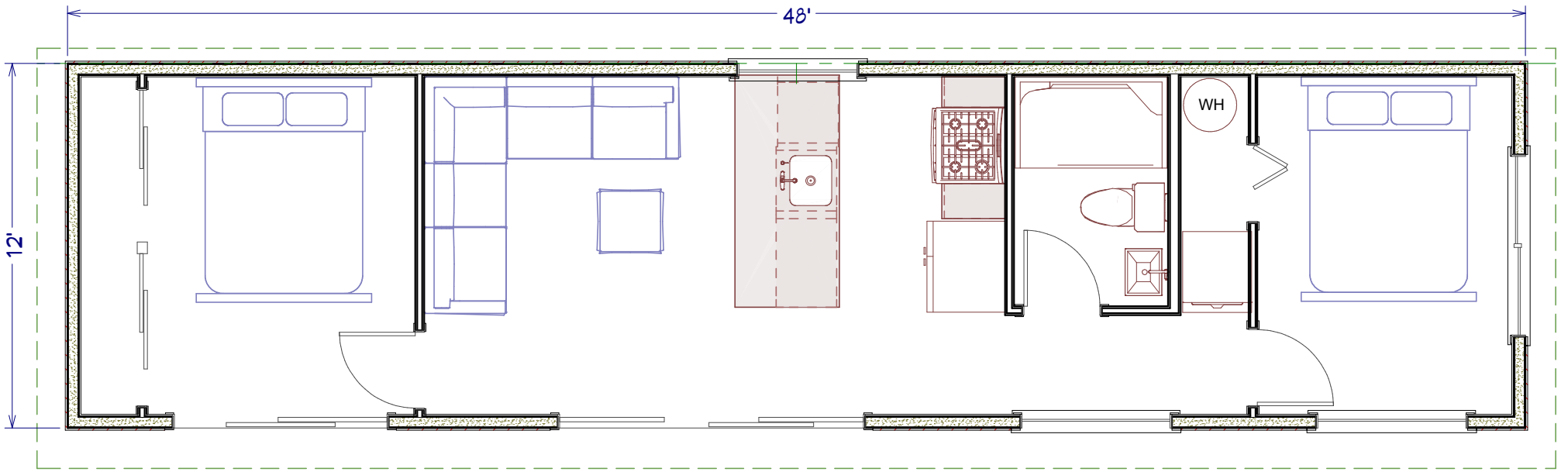
12X48 OUTLOOK 2 BEDROOM, 1 BATH 576 SQ FT
