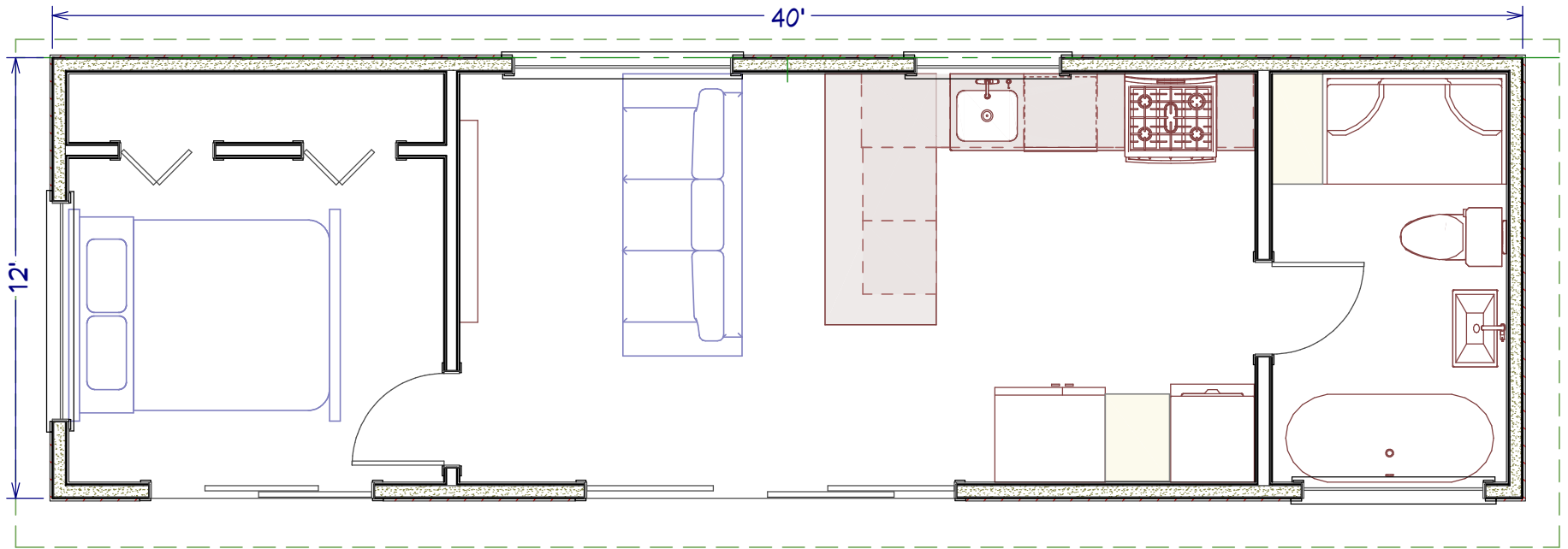
12X40 OUTLOOK 1 BEDROOM, 1 BATH 480 SQ FT
