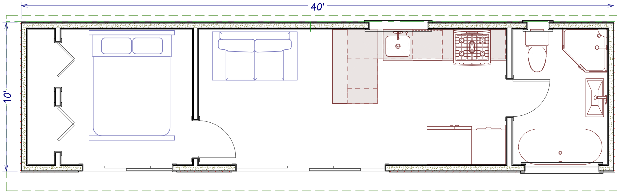
10X40 OUTLOOK 1 BEDROOM, 1 BATH 400 SQ FT
